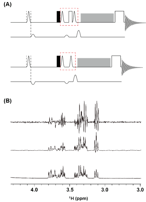
Figure 2. (A) Comparison of modified (upper) and original (lower) iSQC with the adiabatic spinlock (asl). Dashed-boxes indicate differences between modified and original iSQC sequences with asl. (B) Stacked 1D projection spectra of original (upper)/ modified (middle) iSQC spectra and ^1\text{H} NMR spectrum (lower) of D-glucose.
